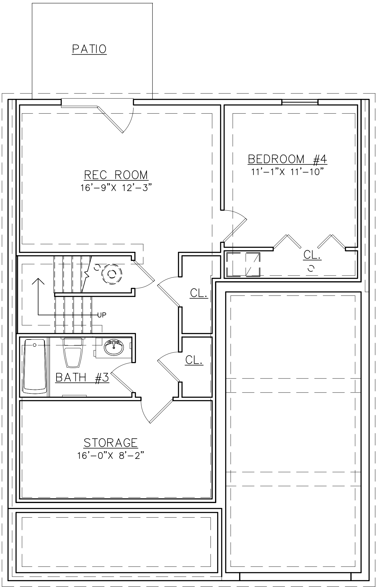
FINSIHED BASEMENT FLOOR PLAN
