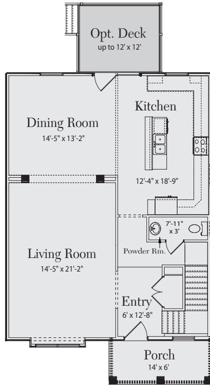
Main Level
