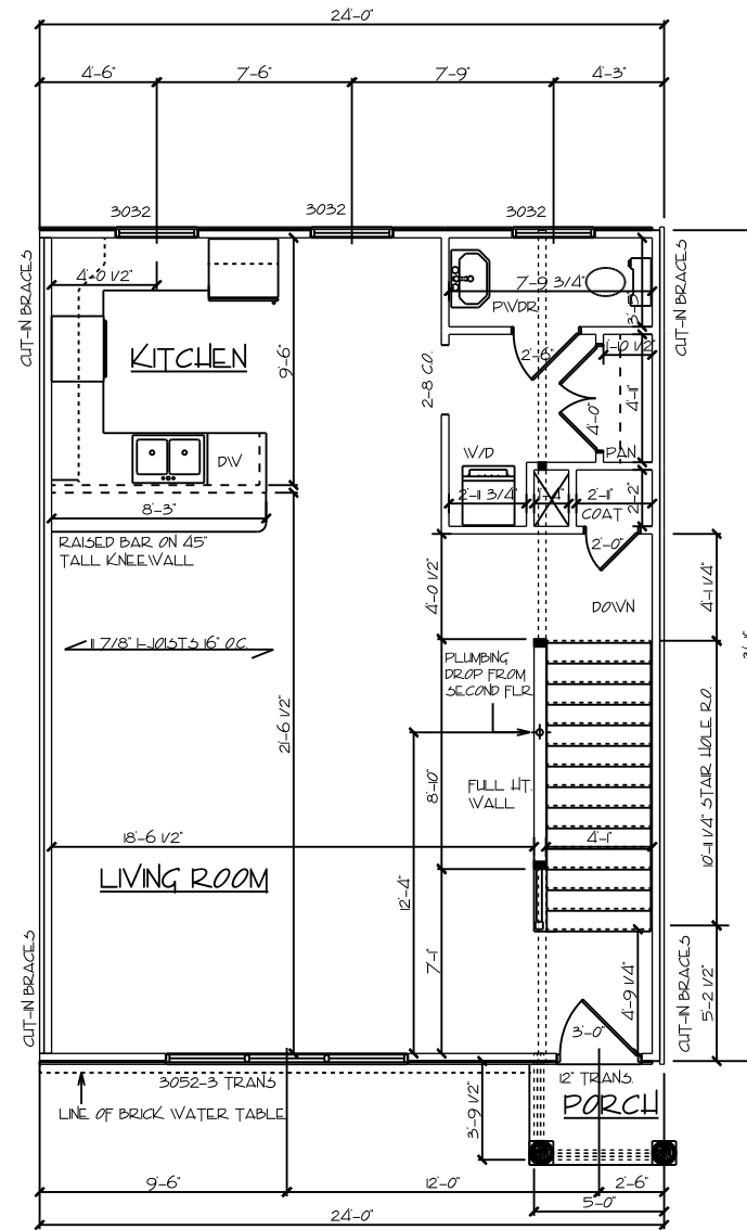
ASHTON DRIVE UNDER 1ST FLOOR PLAN A
