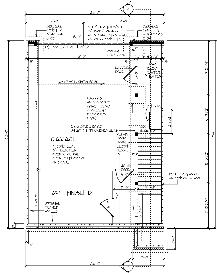
ASHTON DRIVE UNDER FOUNDATION PLAN
