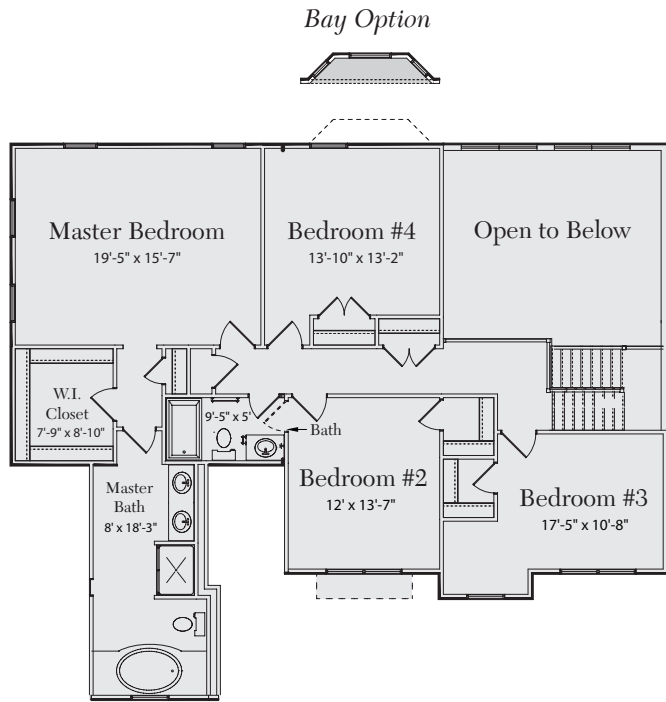
Upper Level
