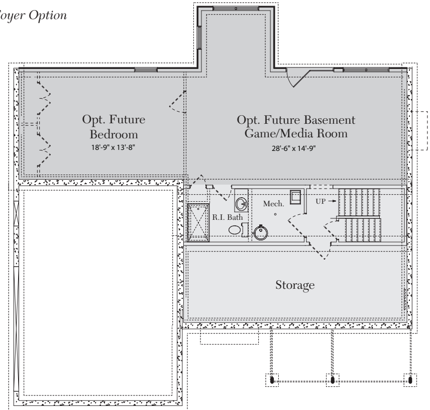
Lower Level
